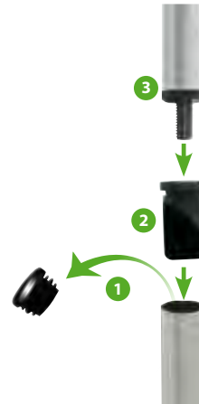
EXTENSION DE PIED D25 - 270 mm 270 mm Leg extension
