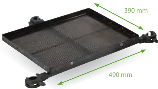
DESSERTER XL ALU 490 x 390 mm Painted alu Side Tray XL - 490 x 390 mm
